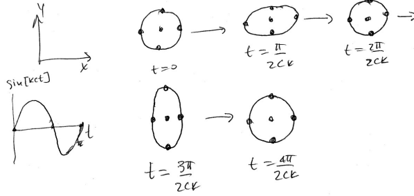
Figure 2: The first of two polarization modes of propagating gravitational waves. This is the plus-polarization where a ring of particles oscillate in the pattenr of a + sign.
