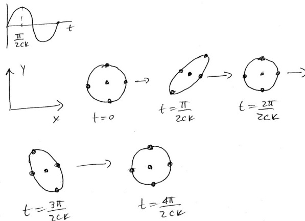
Figure 3: The second of the polarization modes for gravitational waves. This is the cross-polarization where a ring of particles oscillate in the pattern of an \times sign.
